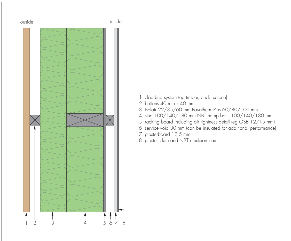
Figure 1 Typical installation showing Isolair or Pavatherm-Plus insulation boards on a timber frame.
